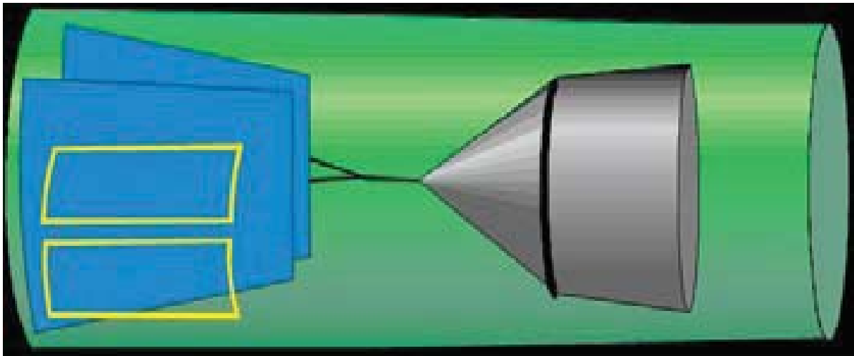
The Modified Jones-Davis BRD. Water flow is left-to-right. Courtesy NOAA Fisheries and Gulf of Mexico Fishery Management Council.
